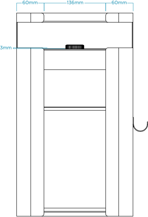
Back dimensions
