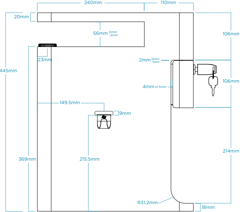
Side dimensions
